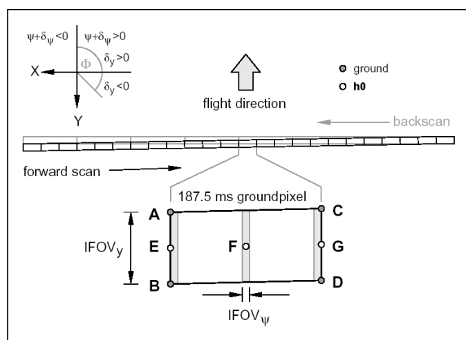
Figure 2: Ground pixel geometry.
